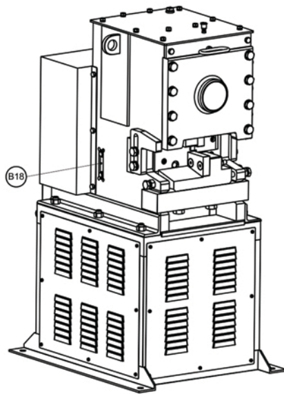
ISO METRIC VIEW
