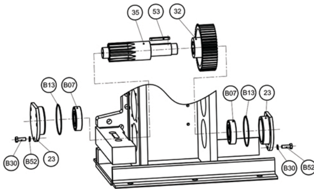
SHAFT GEAR 1 SUB
